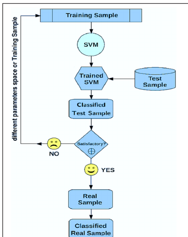
Figure 2. Schematic representation of the SVM algorithm classification process.
