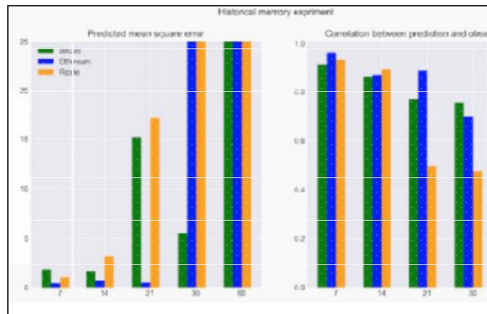
Fig. 4: Performance of LSTM model, given 7, 14, 21, 30, and 60 days price history as input features. Left and right panels represent model-data mean square error and Pearson correlation.
