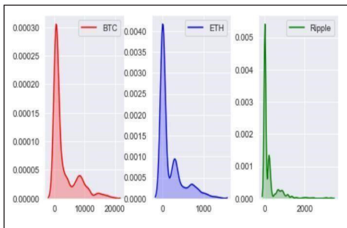
Figure 1: Density distribution of the price history from 7th August 2015 to 2nd June 2018, for Bitcoin (left panel), Ethereum (middle panel), and Ripple (right panel), respectively.
